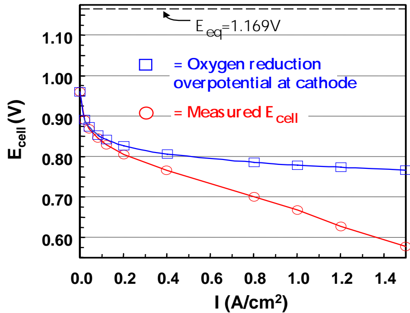
Figure 10 (Lower curve) Cell Voltage ( E_{cell} ) of a State-of-the-art H_2 /Air Membrane Electrode Assembly Operated at 80^\circ\text{C} versus the Current Drawn from the Cell (in \text{amp}/\text{cm}^2 ) (Gasteiger and Mathias 2002) (The equilibrium [theoretical] cell voltage [1.169 V] is shown by the dashed line at the top of the figure.) (Upper curve) Reduction from the Theoretical Value Caused by the Oxygen Reduction Overpotential at the Cathode Alone (Note that the overpotential is large at all but the very lowest currents. The remaining loss in potential at a given current is caused by internal resistance in the cell and to O_2 gas transport limitations through the air in the porous cathode composite.)
