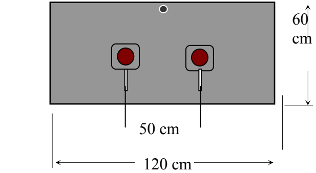
Fig 11: Plan and construction of worktop for cooking
