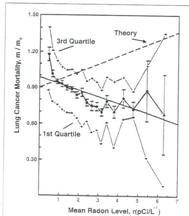
Fig. 5.—Lung cancer mortality rates ( m ) in the United States. Plot data are drawn from [37]. A. Plot shows lung cancer mortality rates (age-adjusted) for males versus average radon level ( r ) in homes in 1729 counties (90% of nation's population). y = year. B. Plot shows lung cancer mortality rates for males from A, corrected for smoking prevalence. C. Plot shows lung cancer mortality rates (age-adjusted) for females versus average radon level ( r ) in homes in 1729 counties (90% of nation's population). y = year. D. Plot shows lung cancer mortality rates for females from C, corrected for smoking prevalence.
