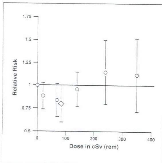
Fig. 4.—Plots show relative risk of mortality from lung cancer versus dose to lung, with 95% confidence limits.
